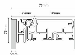
SINGLE SIDED - FRAME I SIMPLE FACE - CADRE I
